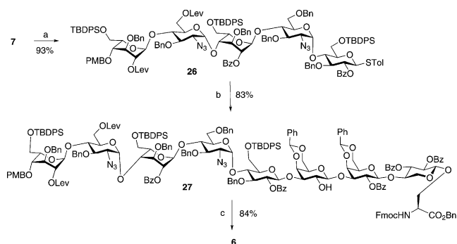
Scheme 3. Reagents and conditions: a) AgOTf, p -TolSfCl, 4 Å M.S., -78^{\circ}\text{C} , then 8 , TTBP, -78^{\circ}\text{C} – 0^{\circ}\text{C} ; b) AgOTf, p -TolSfCl, 4 Å M.S., -78^{\circ}\text{C} , then 9 , TTBP, -78^{\circ}\text{C} – 0^{\circ}\text{C} ; c) 1. HF/pyridine; 2. TEMPO, BAIB, \text{CH}_2\text{Cl}_2/\text{H}_2\text{O}/t\text{BuOH} (4:1:4); 3. MeI, \text{K}_2\text{CO}_3 , DMF. BAIB = [bis-(acetoxy)iodo]benzene, DMF = N,N' -dimethylformamide, TEMPO = 2,2,6,6-tetramethyl-1-piperidinyl-oxyl.
