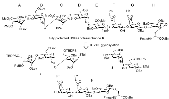
Figure 1. Retrosynthetic analysis of octasaccharide amino ester 6 . Bn = benzyl, Bz = benzoyl, Fmoc = 9-fluorenylmethoxycarbonyl, Lev = levulinoyl, PMB = para -methoxybenzyl, TBDPS = tert -butyldiphenylsilyl, STol = thiotolyl.
