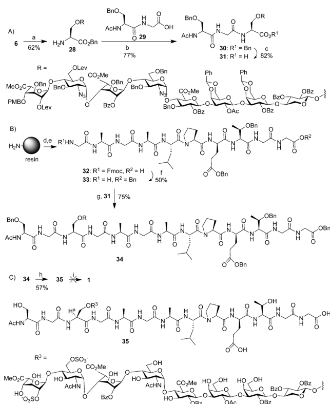
Scheme 4. Reagents and conditions: a) 1. \text{Ac}_2\text{O} , pyridine, 50^{\circ}\text{C} ; 2. piperidine, \text{CH}_2\text{Cl}_2 ; b) HATU, DIPEA, DMF; c) Pd/C, \text{H}_2 , \text{NH}_4\text{OAc} , \text{CH}_2\text{Cl}_2/\text{MeOH} (1:1); d) multiple rounds of automated solid phase peptide synthesis; e) TFA/ \text{H}_2\text{O} /Phenol/TIPS; f) 1. BnBr, DIPEA, DMF; 2. piperidine, DMF; g) HATU, DMF; h) 1. Zn, \text{CuSO}_4 (sat.), \text{Ac}_2\text{O}/\text{THF}/\text{HOAc} ; 2. \text{NH}_2\text{NH}_2\cdot\text{H}_2\text{O} , HOAc, \text{CH}_2\text{Cl}_2/\text{MeOH} (1:1); 3. \text{SO}_3\cdot\text{Et}_3\text{N} , DMF, 55^{\circ}\text{C} ; 4. \text{H}_2 , Pd/C, \text{CH}_2\text{Cl}_2/\text{MeOH} (1:1); i) base-catalyzed hydrolysis. DIPEA = diisopropylethylamine, HATU = O -(7-azabenzotriazol-1-yl)- N,N,N',N' -tetramethyluronium hexafluorophosphate, TFA = trifluoroacetic acid, TIPS = triisopropylsilane, THF = tetrahydrofuran.
